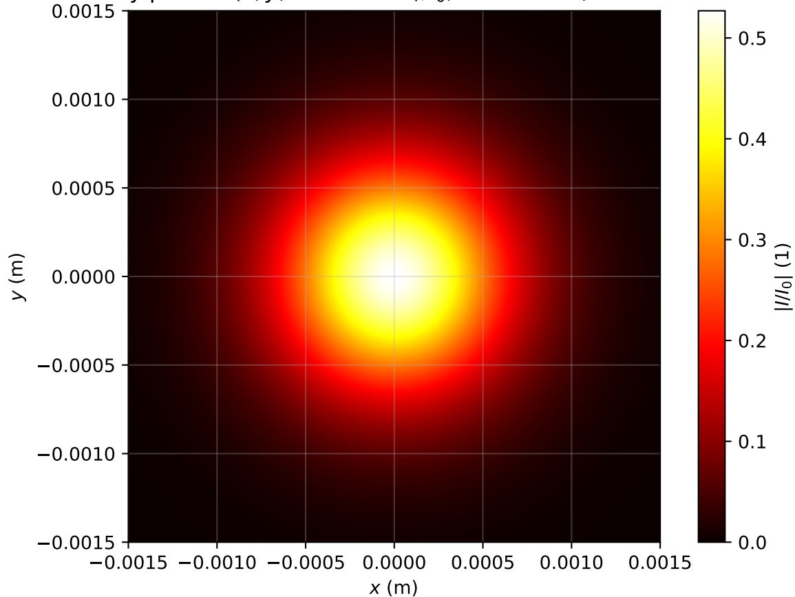
Intensity profile I(x, y, z = 3.184m)/I_0 , \text{Pin}=0.5\text{Pcr} , artificial time
